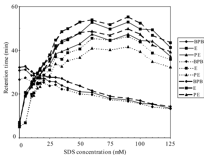
Figure 2. Effect of SDS concentrations on retention times with different columns.
