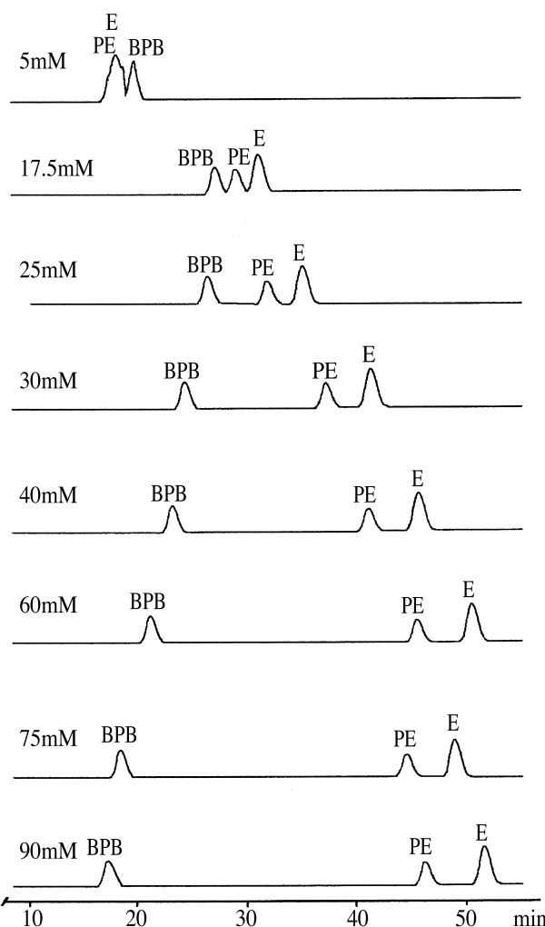
Figure 4. HPLC chromatograms with different SDS concentrations. (Merck)
