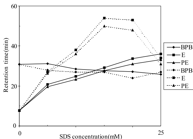
Figure 3. Effect of different brands' SDS on retention times. (—: SDS from Merck; .....: SDS from Sigma)
