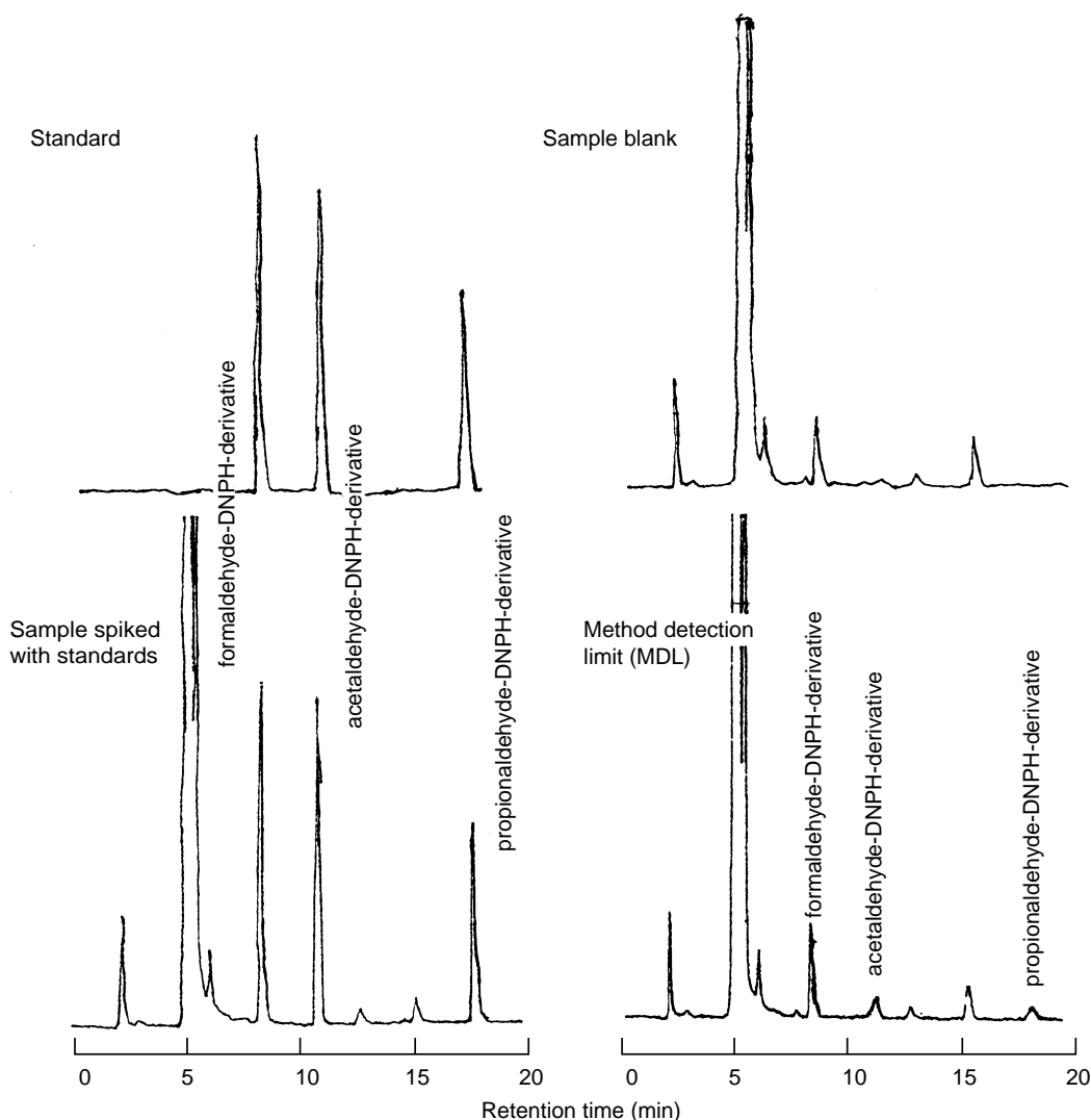
Figure 6. HPLC chromatograms of formaldehyde, acetaldehyde and propionaldehyde DNPH derivatives in D.I. water. A mobile phase of \text{CH}_3\text{CN}/\text{H}_2\text{O} = 55 / 45 (v / v) with flow rate at 1 mL/min and UV detection at 360nm was used. Concentration of standard solution was 1 ppm and ample spiked with 100 ppb standard and 1 ppb MDL.
