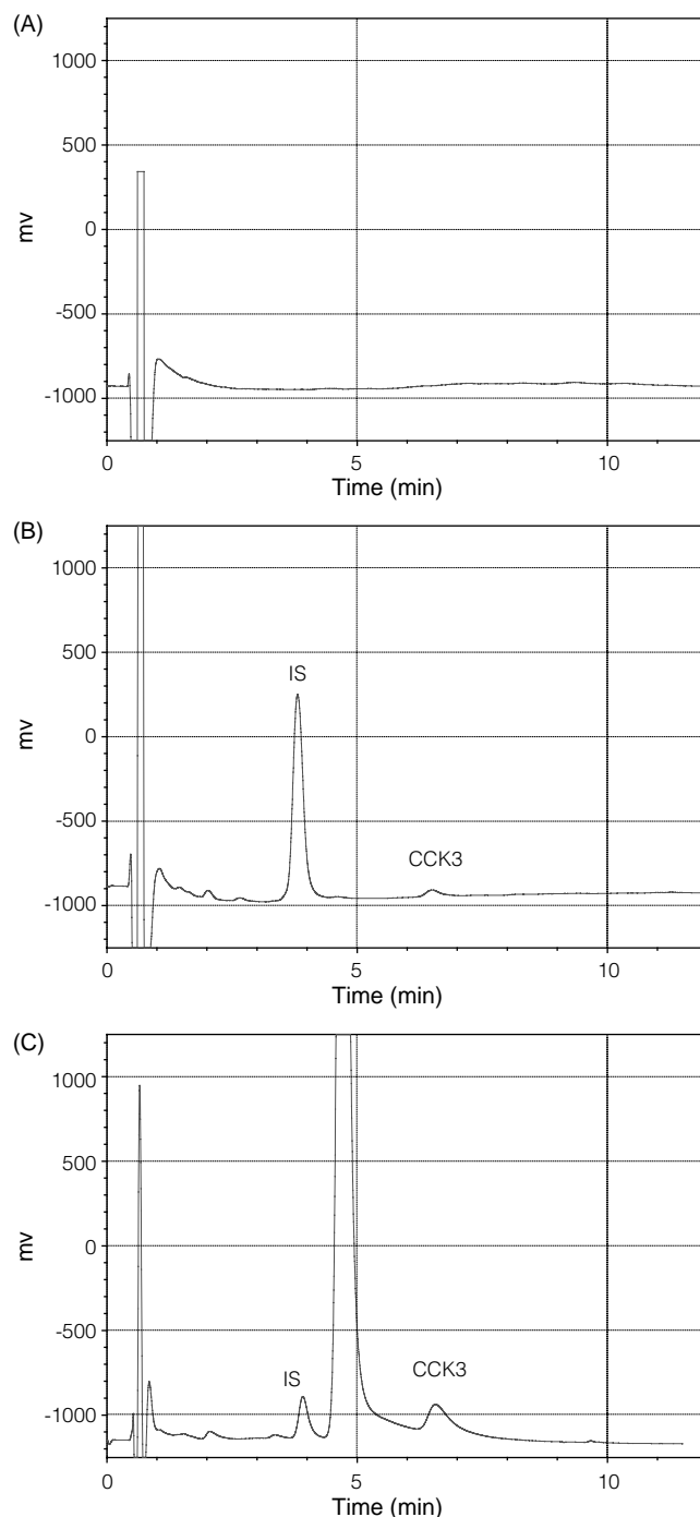
Figure 2. HPLC chromatograms of CCK3 in rat plasma. (A) blank plasma (B) plasma spiked with CCK3 (10 ng/mL) and internal standard (IS) (1 \mu g/mL) (C) rat plasma extracted for 5 min after IV administration of 3.97 mg/kg of CCK3.
