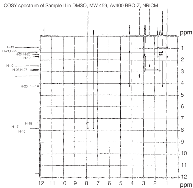
Figure 5. 1 H- 1 H COSY spectrum of vardenafil analogue (A).
