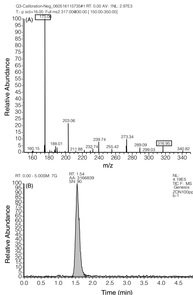
Figure 3. LC/ESI-MS-MS product ion spectra in the negative mode (A) and total ion chromatogram (B) of ZON (100 ppb)
