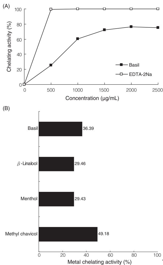
Figure 2. Metal chelating activity of basil essential oil and its major components. (A) Concentration dependency of the metal chelating activity of basil essential oil and EDTA-2Na. (B) Metal chelating activity of three major chemical components of basil compared with its essential oils at the concentration of 1 mg/mL.
