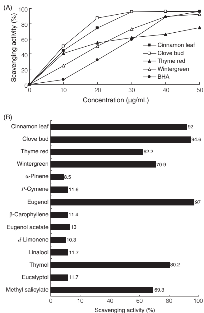
Figure 1. ABTS •+ radical scavenging activity of the top four essential oils with the highest activity and their major components. (A) Concentration-dependent effect of ABTS •+ radical scavenging activity of cinnamon leaf, clove bud, thyme red, wintergreen essential oils and BHA. (B) ABTS •+ radical scavenging activity of major chemical components of cinnamon leaf, clove bud, thyme red, wintergreen compared with its essential oils at the concentration of 30 µg/mL.
