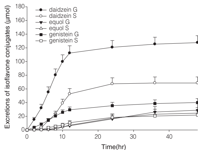
Figure 3. Mean ( \pm SE) cumulative urinary recoveries of glucuronides (G) and sulfates (S) of daidzein, equol and genistein after intake of 800 mL soymilk in nine adults.
