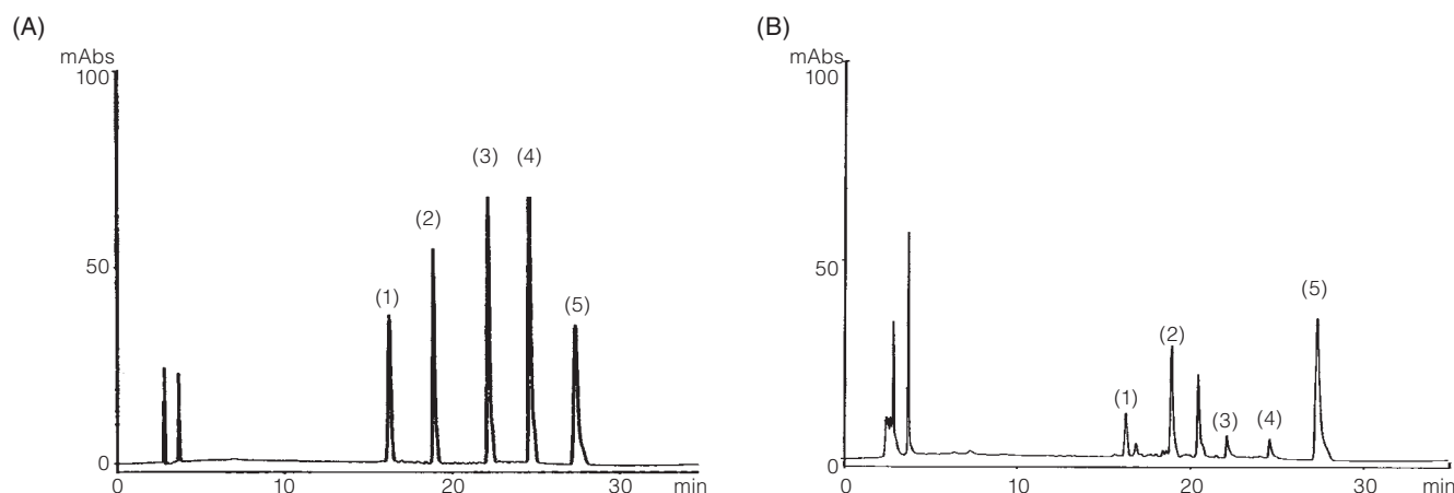
Figure 1. Chromatograms of standards (12.5 \mu\text{g/mL} ) in methanol (A) and soymilk sample (B). 1: daidzin (16.5 min), 2: genistin (19.5 min), 3: daidzein (22.0 min), 4: genistein (24.9 min), 5: 5,7-dimethoxycoumarin (internal standard, 27.5 min).
