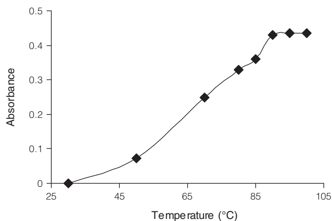
Figure 4. Effect of temperature on the absorbance of INH at 3 \mu\text{g}/\text{mL} .
