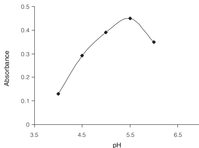
Figure 2. Effect of pH on the absorbance of INH at 3 \mu\text{g}/\text{mL} .
