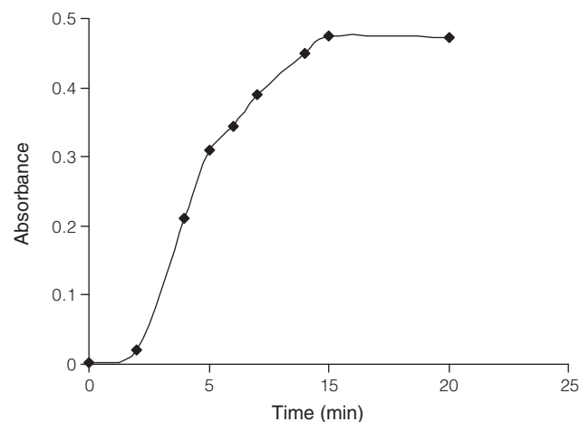
Figure 3. Time course of color development of INH at 3 \mu\text{g}/\text{mL} .
