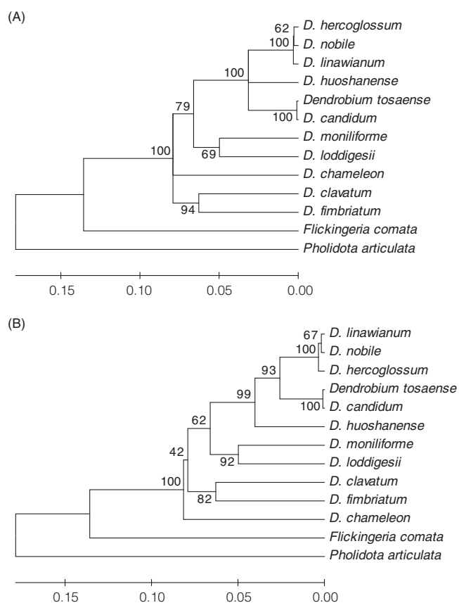
Figure 2. Phylogenetic trees based on the ITS sequence by (A) Neighbor-Joining (NJ) and (B) Maximum Parsimony (MP) methods.
