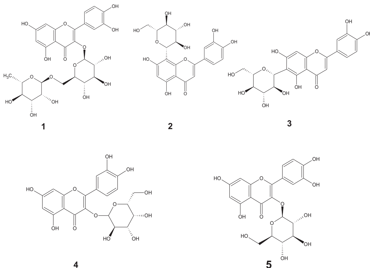
Figure 2 – Structure of bioactive compounds isolated from Nelumbo nucifera seed embryo: rutin (1), orientin (2), isoorientin (3), isoquercetrin (4), and hyperoside (5).
