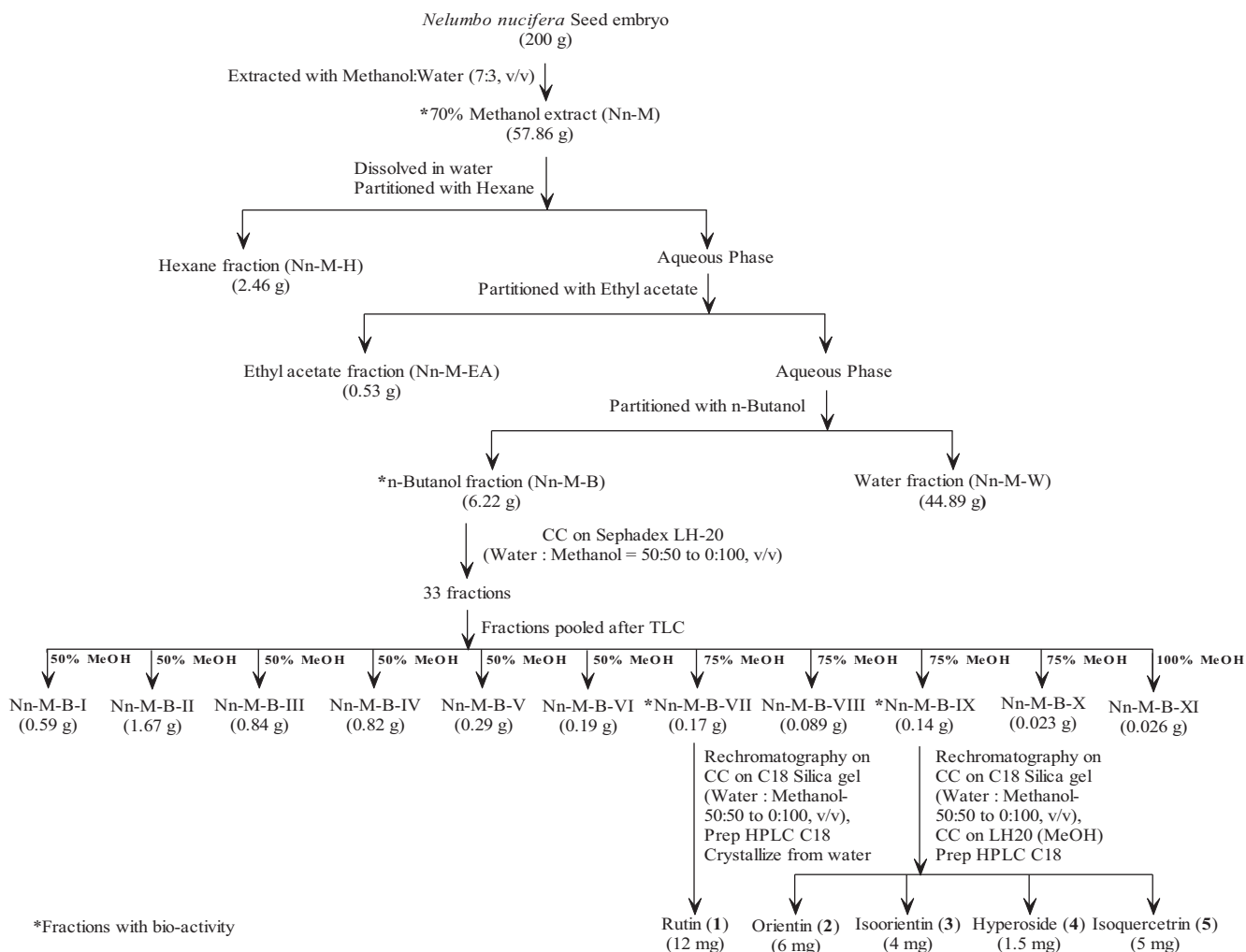
Figure 1 – Extraction and fractionation scheme of Nelumbo nucifera seed embryo. CC = Column Chromatography ;HPLC = high-performance liquid chromatography; TLC = thin-layer chromatography.
