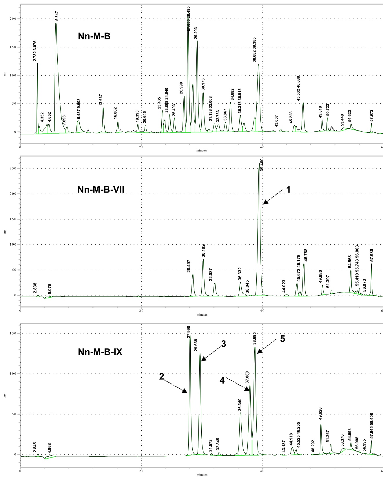
Figure 3 – Typical HPLC profile of the most active fractions of Nelumbo nucifera seed embryo. Rutin (1), orientin (2), isorientin (3), isoquercetrin (4), and hyperoside (5) were detected at 254 nm. HPLC = high-performance liquid chromatography.
